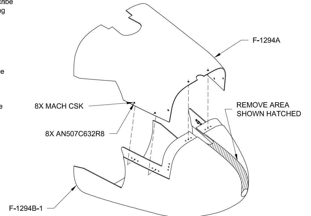
FIGURE 3: F-1294 ASSEMBLY
