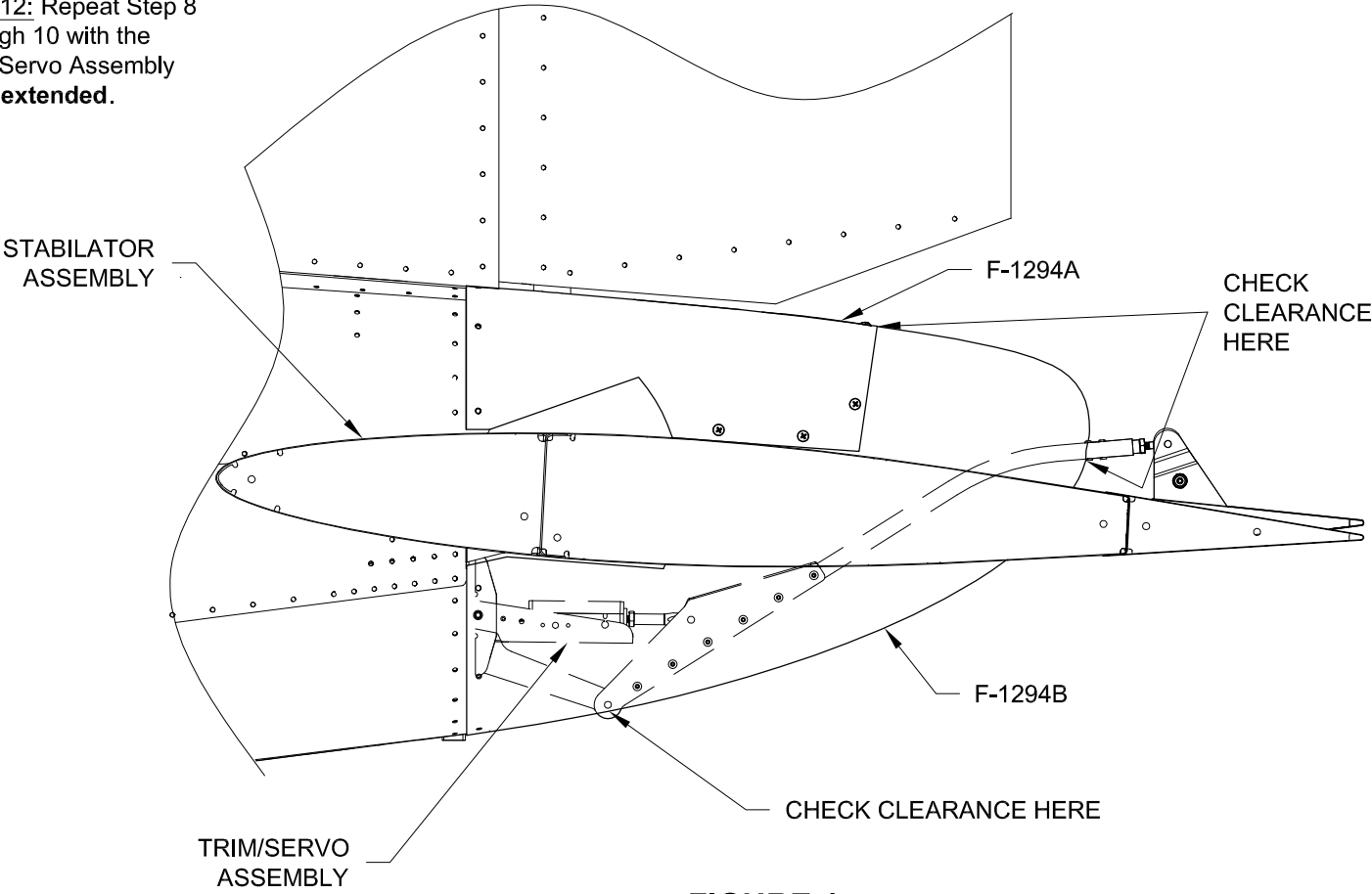
FIGURE 4: TRIM/SERVO CLEARANCE
