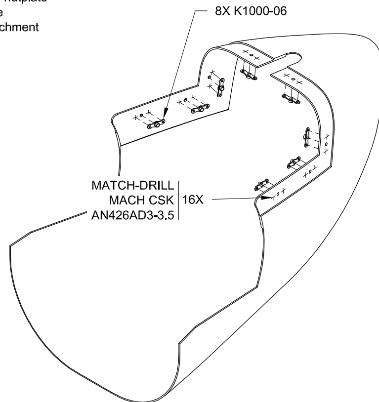
FIGURE 1: F-1294B-1 NUTPLATE INSTALLATION
