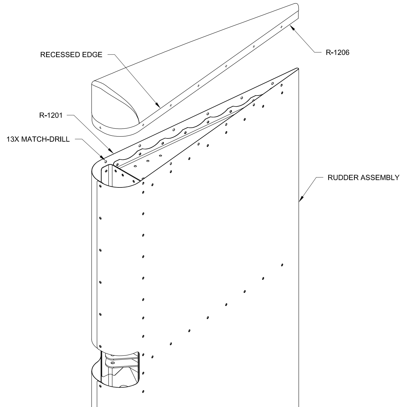
FIGURE 4: RUDDER TIP FAIRING
