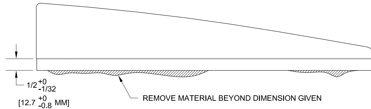
FIGURE 2: R-1206 RUDDER TIP FAIRING
