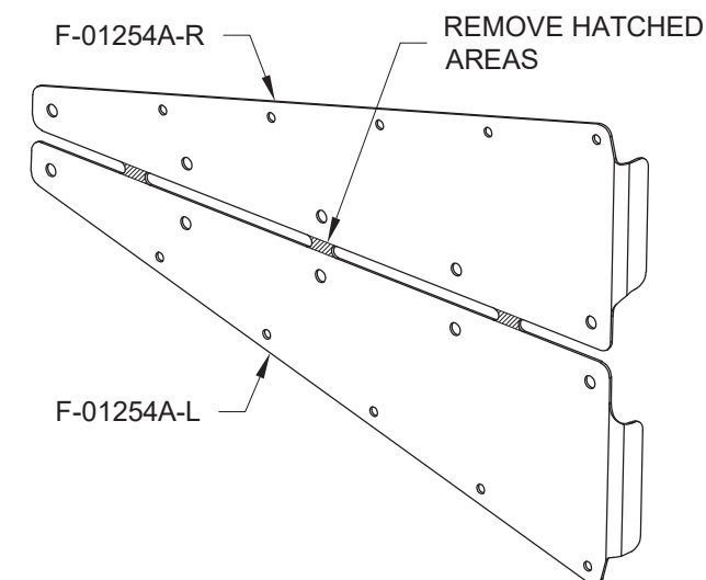
FIGURE 5: SEPARATING THE F-01254A
