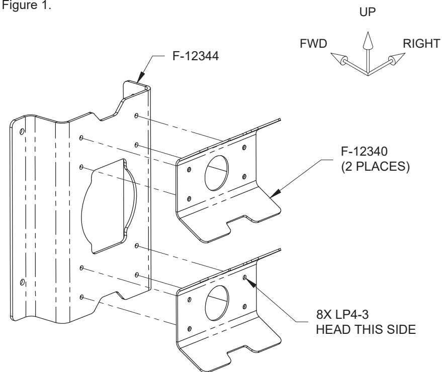
FIGURE 1: FUEL PUMP BRACKET ASSEMBLY
