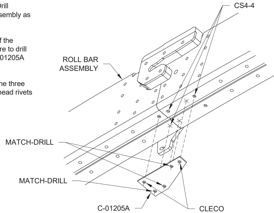
FIGURE 1: DRILLING FOR THE CANOPY LATCH BLOCK
