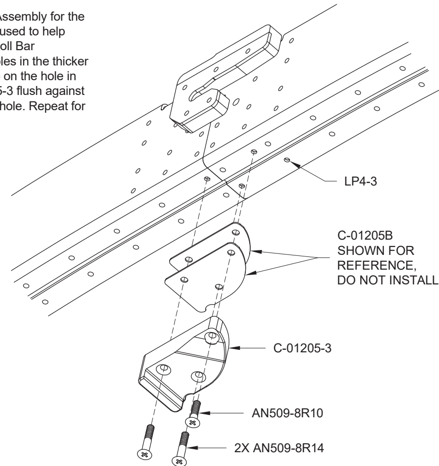
FIGURE 2: C-01205-3 INSTALL
