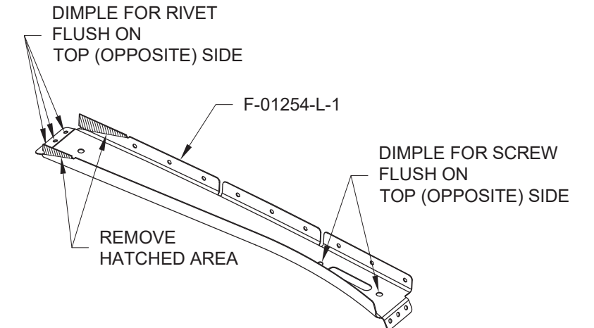
FIGURE 4: TRIMMING THE F-01254-L-1 & -R-1
