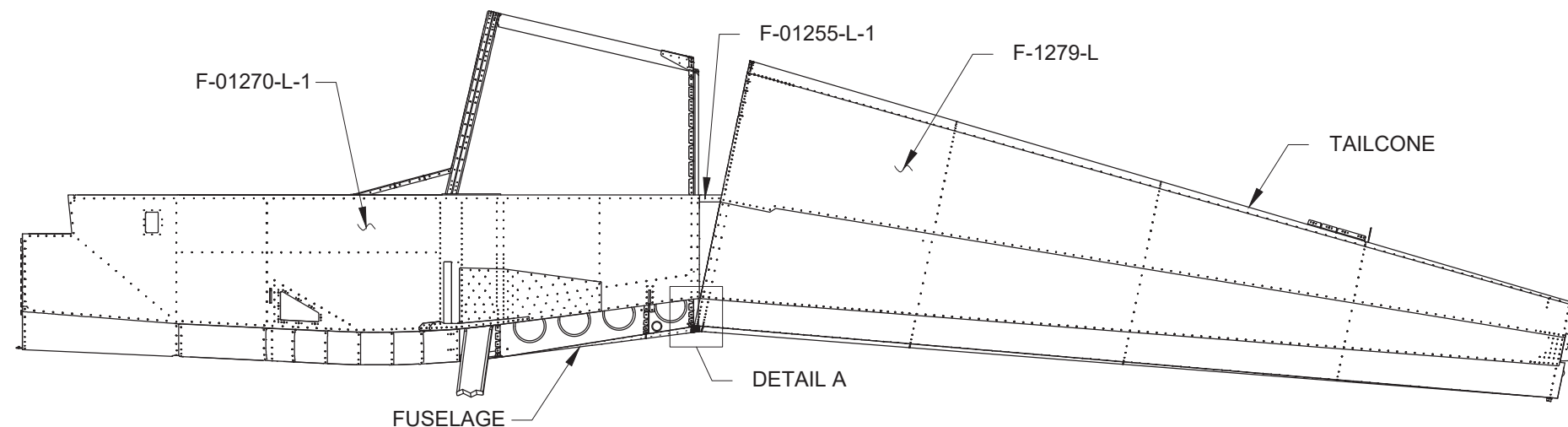
FIGURE 1: TAILCONE ATTACH
