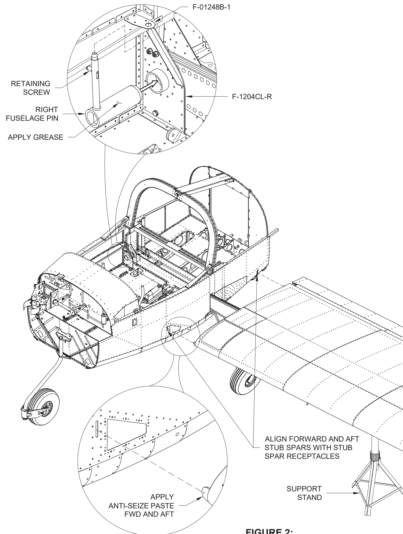
FIGURE 2: WING INSTALLATION
