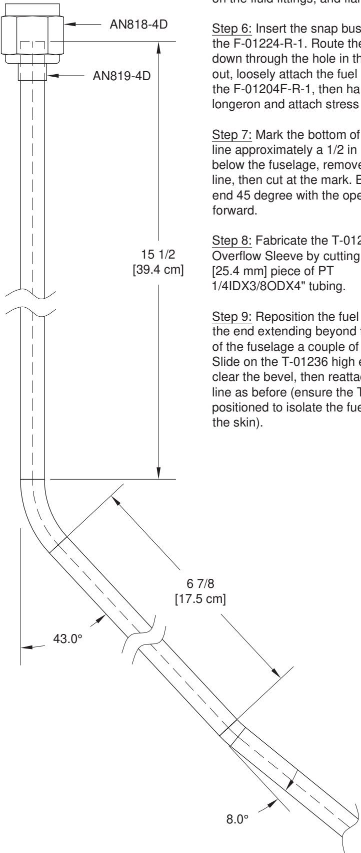
FIGURE 3: T-01235 OVERFLOW FUEL LINE
