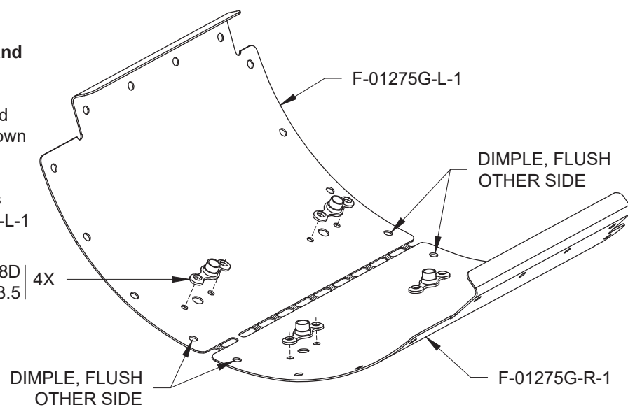
FIGURE 2: PREPARING THE F-01275G-L-1 & -R-1 COVER PLATES
