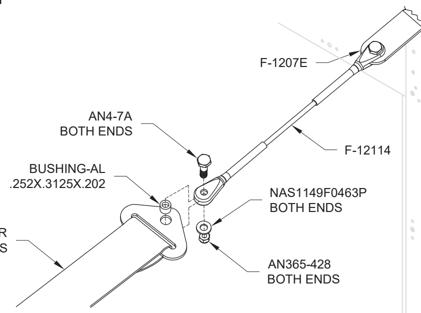
FIGURE 1: SHOULDER HARNESS ATTACH
