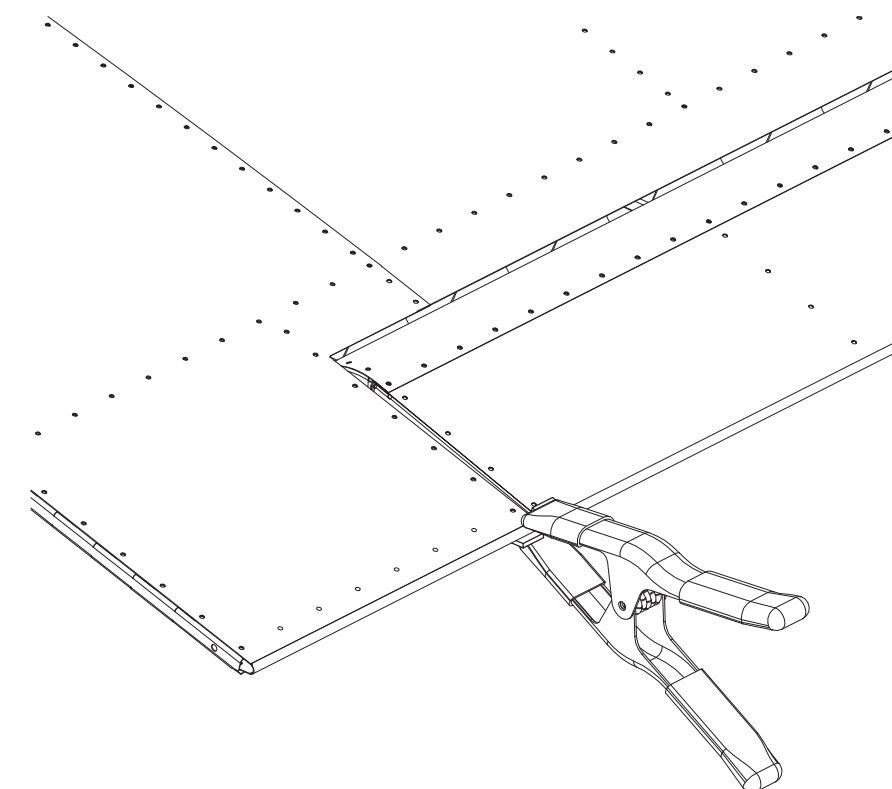
FIGURE 3: SHIMMING & CLAMPING THE FLAPERON TRAILING EDGES (LEFT SIDE SHOWN)
