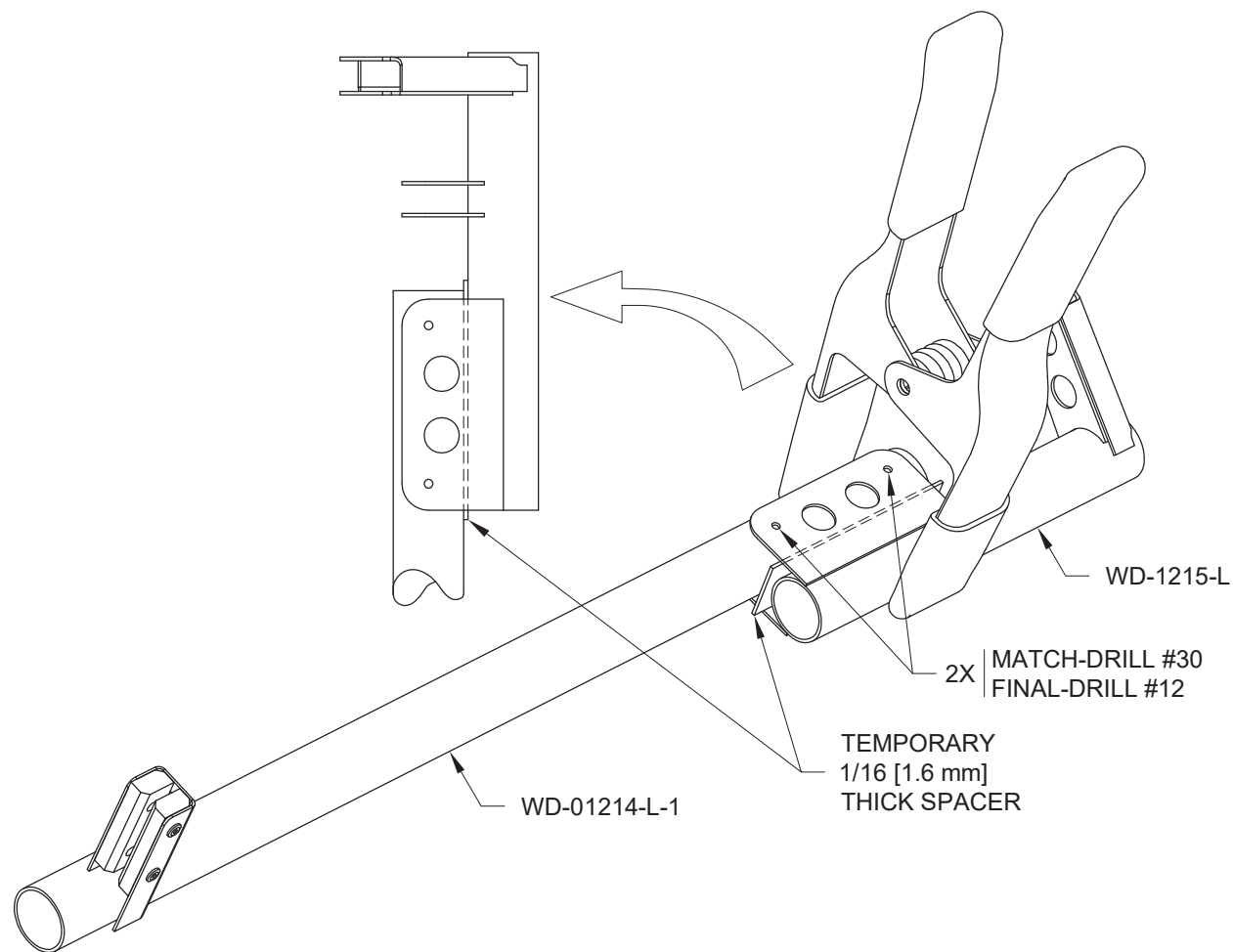
FIGURE 1: DRILLING THE FLAPERON TORQUE TUBES
