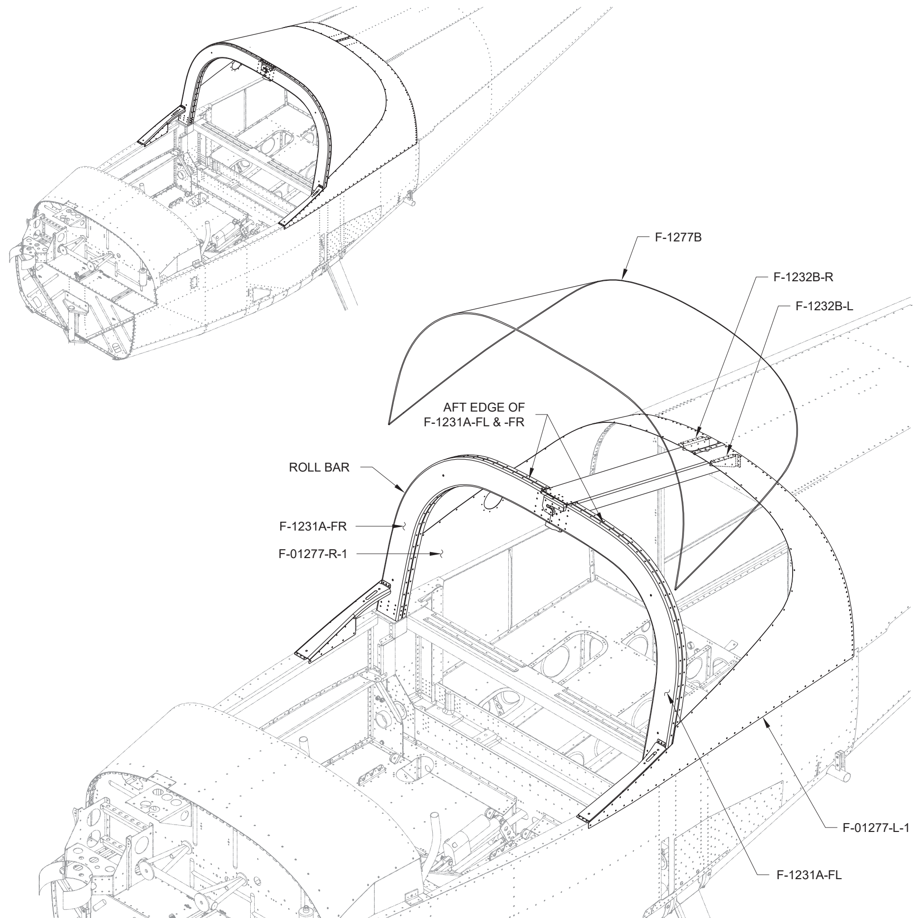
FIGURE 1: AFT WINDOW FIT
