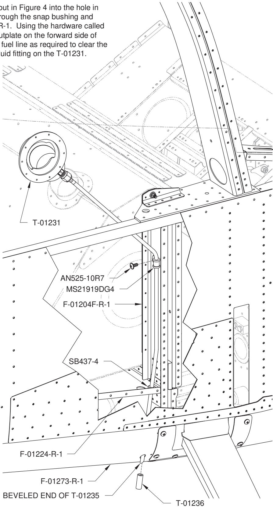
FIGURE 4: OVERFLOW FUEL LINE
