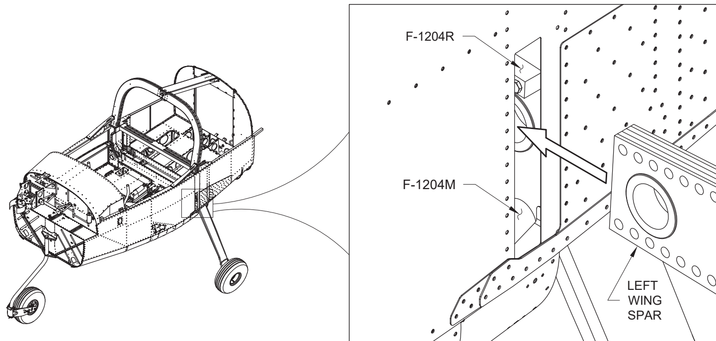
FIGURE 1: WING SPAR RECEPTACLE
