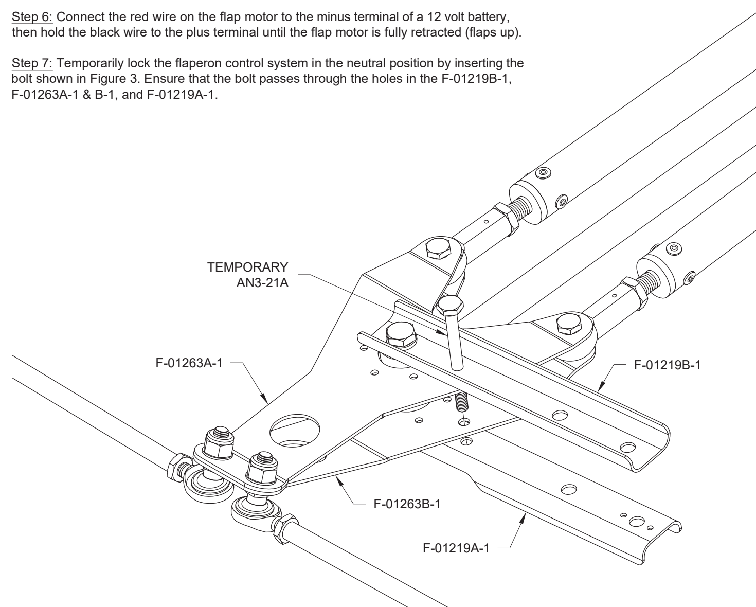
FIGURE 3: LOCKING THE FLAPERON CONTROL SYSTEM
