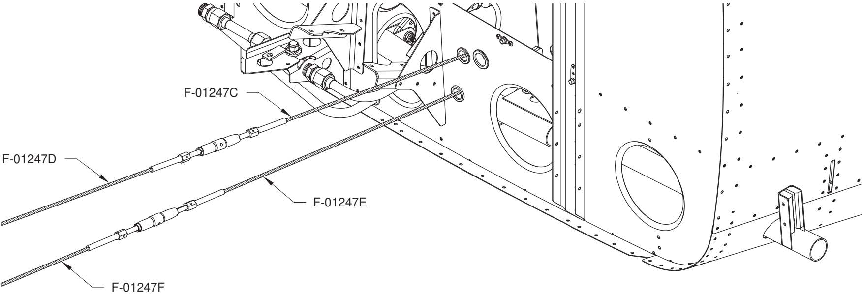
FIGURE 2: STABILATOR CABLES
