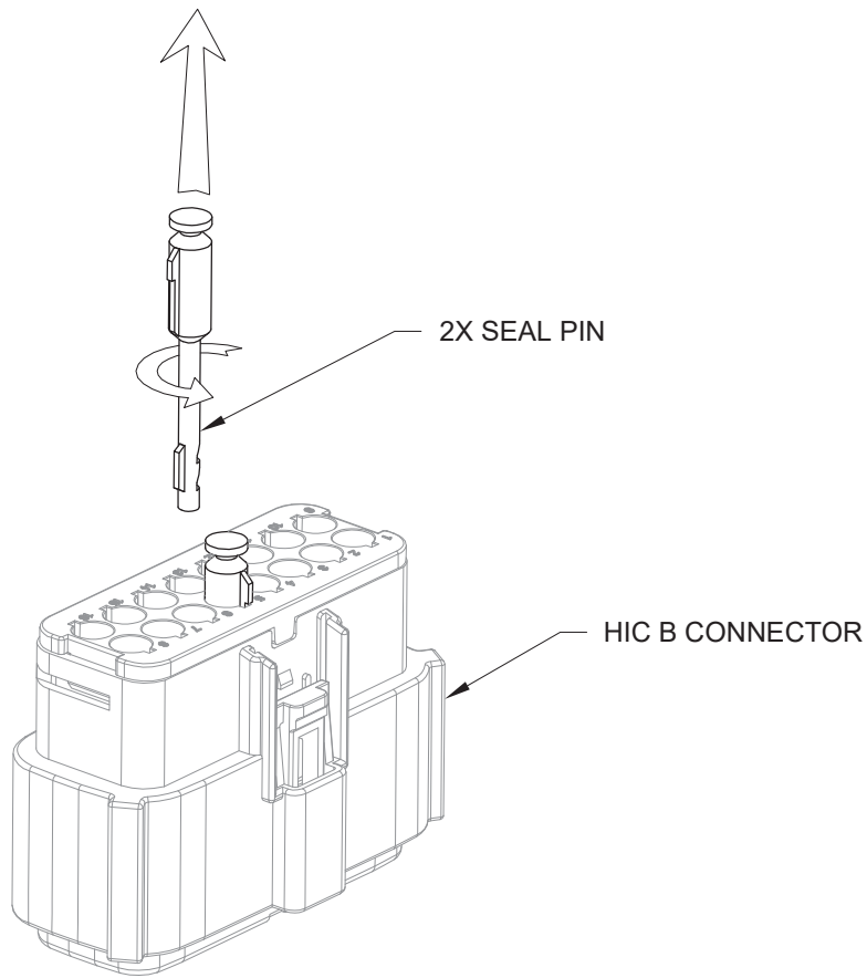
FIGURE 1: REMOVING SEAL PINS (WIRES NOT SHOWN FOR CLARITY)
