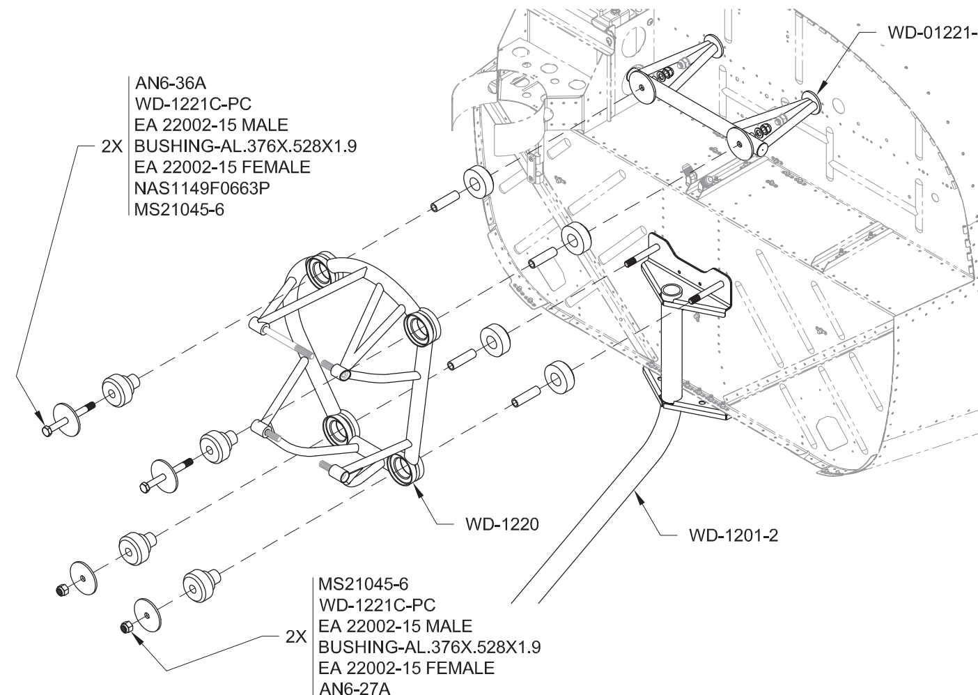
FIGURE 3: ATTACH ENGINE TO FUSELAGE (ENGINE NOT SHOWN)
