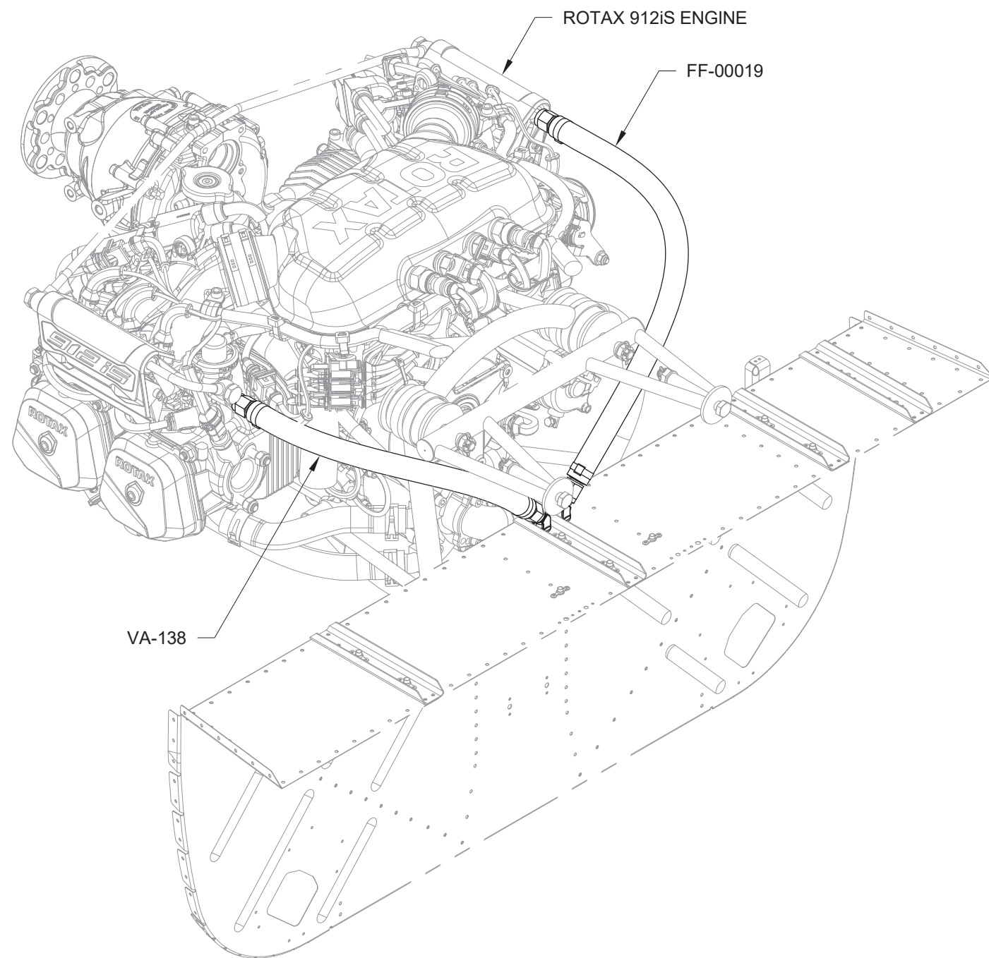
FIGURE 1: CONNECT FUEL HOSES TO ENGINE
