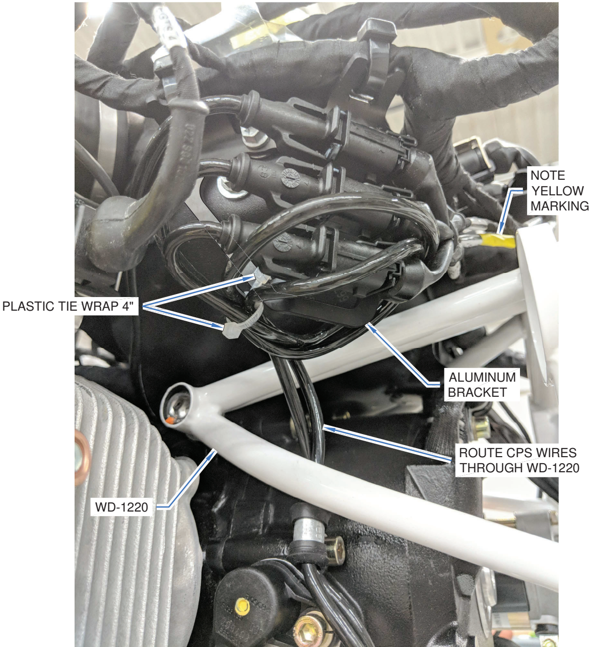
FIGURE 2: ROUTE & SECURE CPS WIRES
