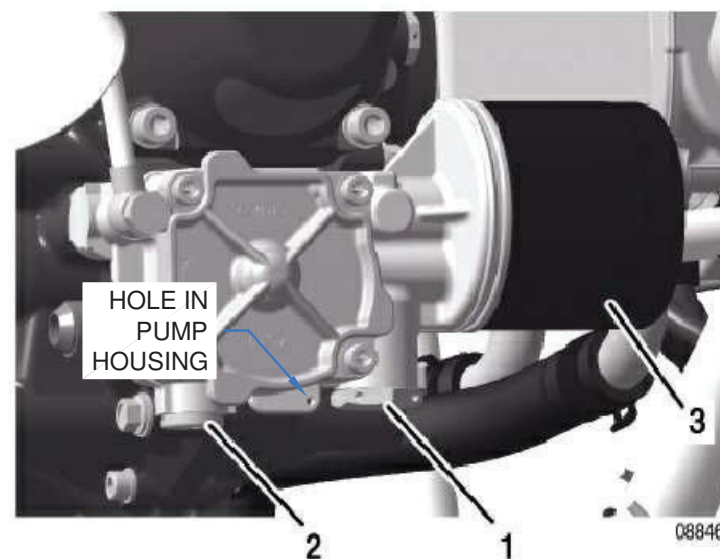
FIGURE 3: OIL PRESSURE REGULATOR PLUG LOCATION
