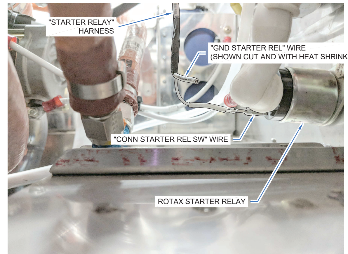
FIGURE 3: ROTAX STARTER RELAY
