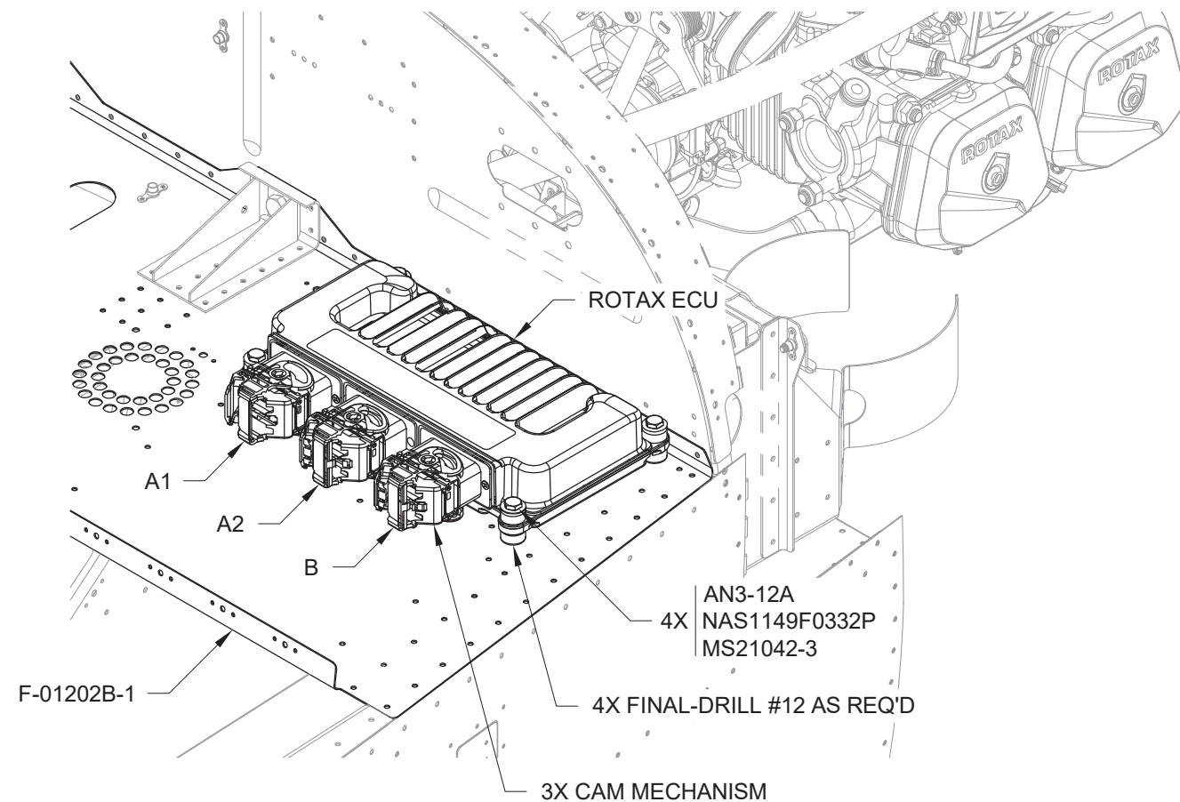
FIGURE 1: ENGINE CONTROL UNIT (ECU) INSTALLATION
