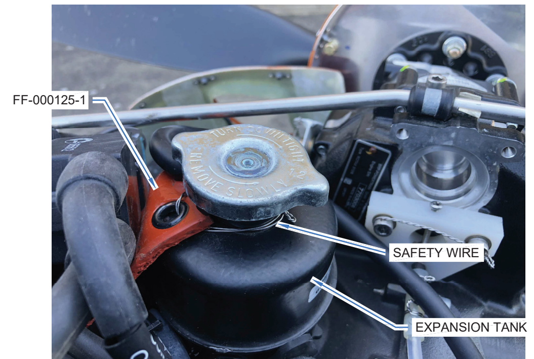
FIGURE 4: EXPANSION TANK SAFETY WIRE (AFT VIEW LOOKING FORWARD)
