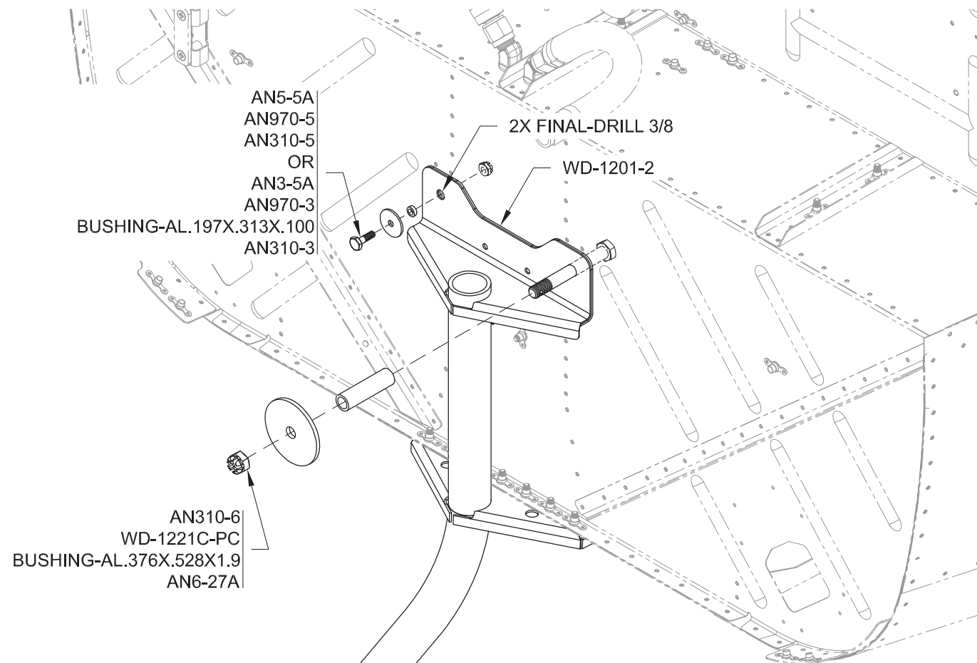
FIGURE 1: FINAL-DRILL NOSE GEAR FLANGE
