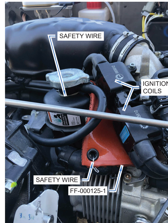
FIGURE 2: IGNITION COILS FIRE SLEEVE (TOP VIEW LOOKING DOWN/AFT)
