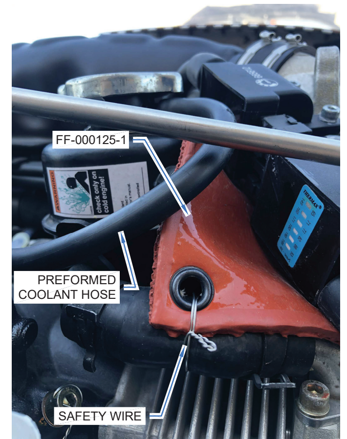
FIGURE 3: COOLANT HOSE SAFETY WIRE (FRONT VIEW LOOKING AFT)
