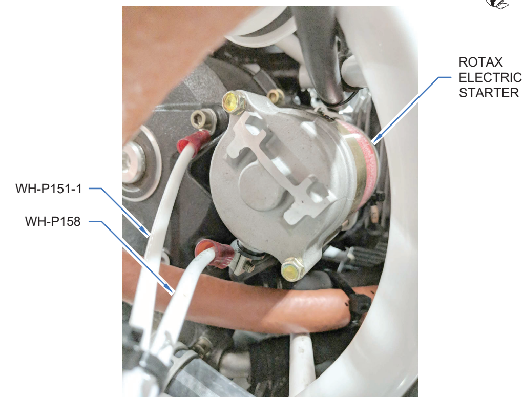
FIGURE 2: ROTAX ELECTRIC STARTER
