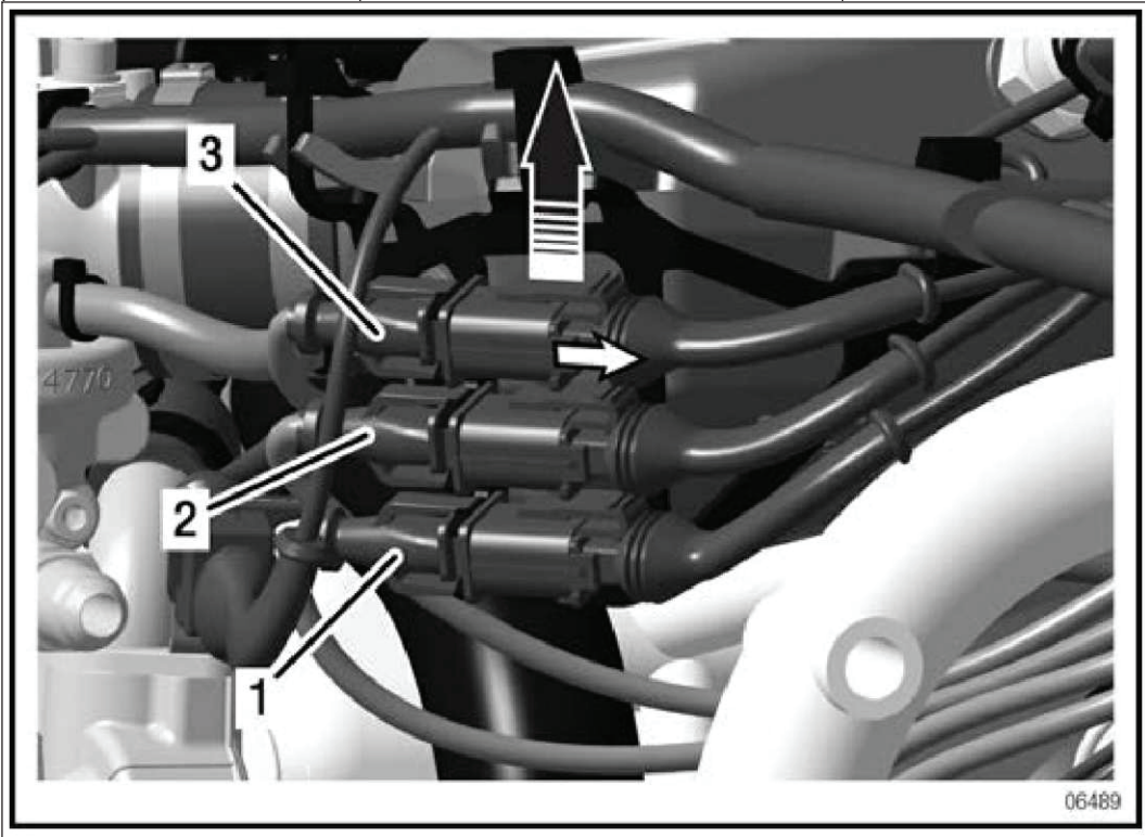
FIGURE 2: PREFORMED RADIATOR OUTLET HOSE & CPS CONNECTORS
