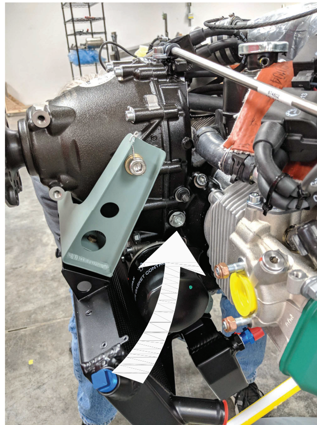
FIGURE 1: MAGNETIC PLUG LOCATION
