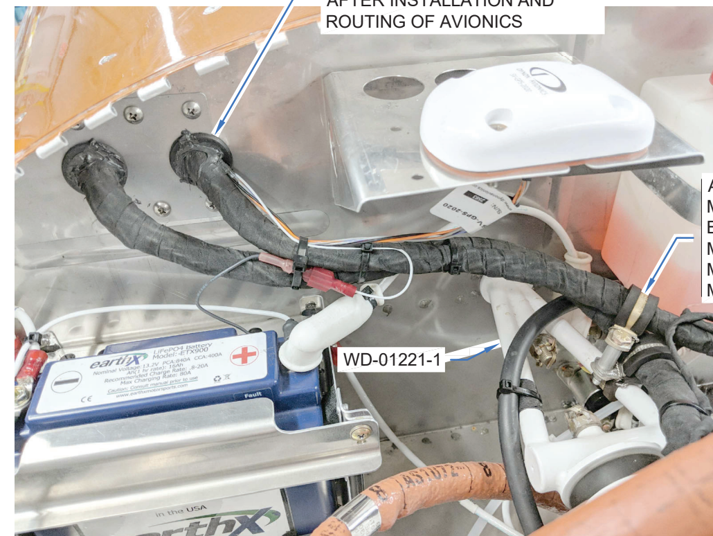
FIGURE 3: ECU CABLE ROUTING - FIREWALL FORWARD (SOME ITEMS SHOWN ARE NOT YET INSTALLED)
