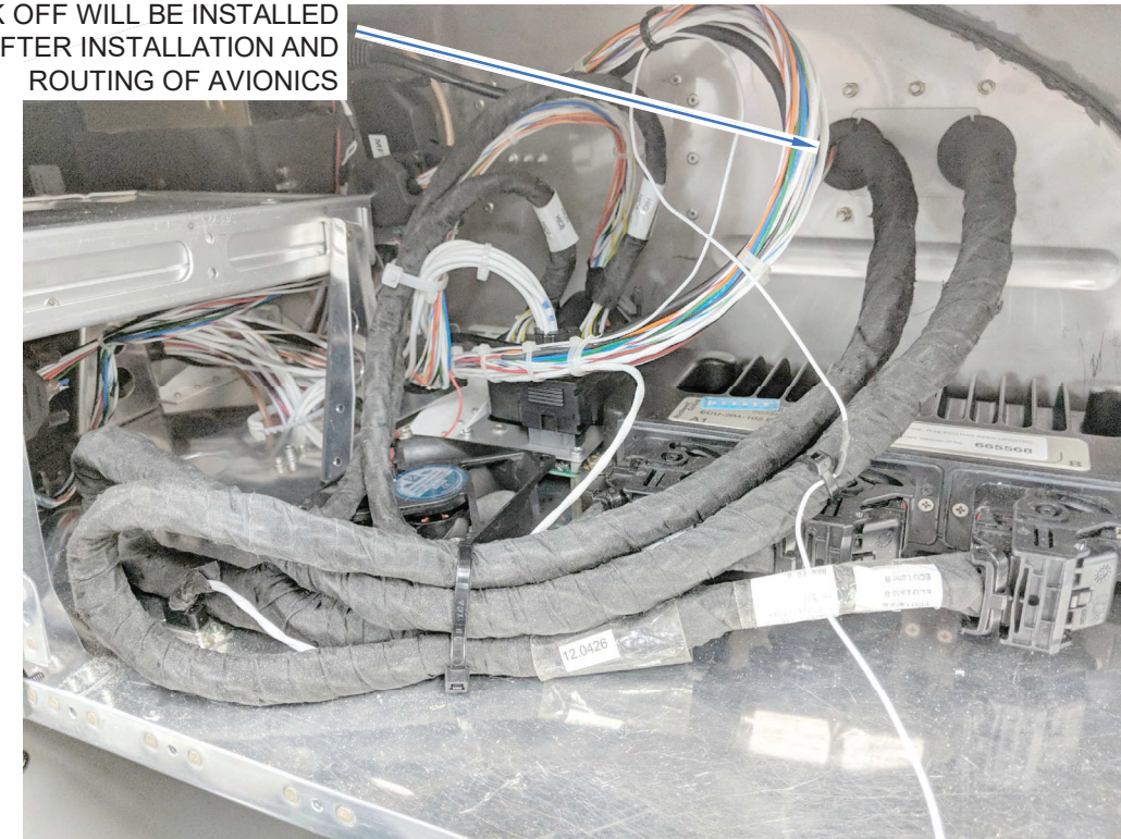
FIGURE 2: ECU CABLE ROUTING - FIREWALL AFT (SOME ITEMS SHOWN ARE NOT YET INSTALLED)
