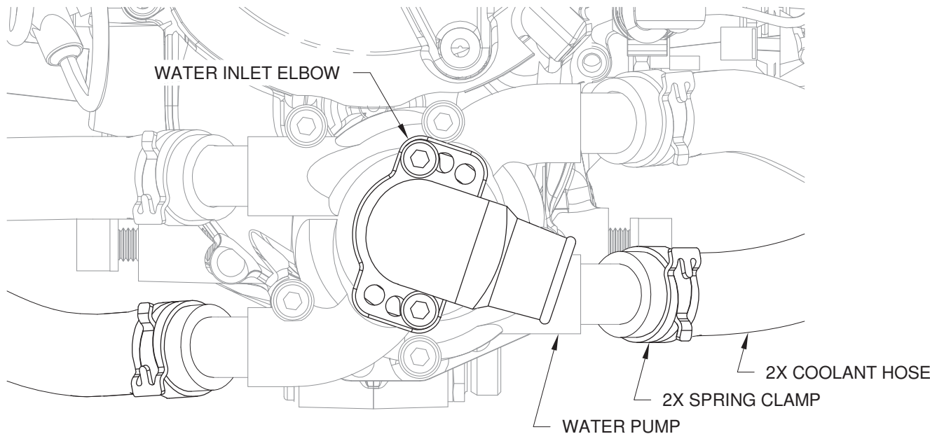
FIGURE 1: WATER INLET ELBOW CLOCKING (AFT VIEW LOOKING FORWARD)
